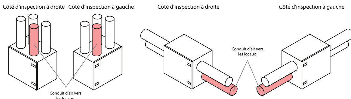
Fig. 3. Classification of units by inspection side
